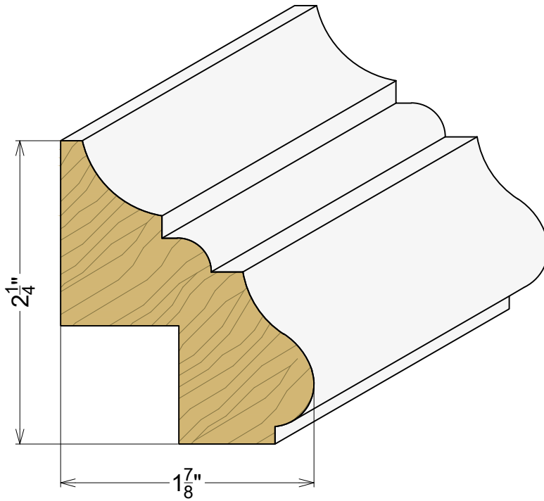
AP 6207 1-7/8" x 2-1/4"
