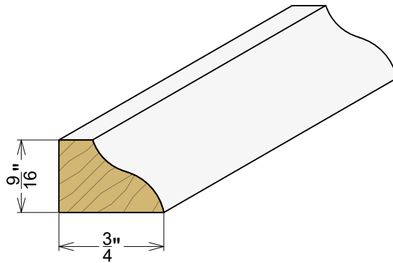
AP 6218 9/16" x 3/4"
