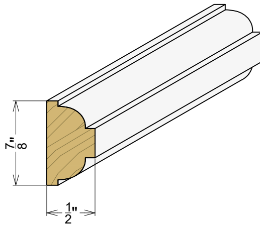
AP 6250 1/2" x 7/8"
