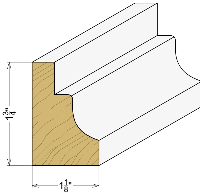
AP 6279 1-1/8" x 1-3/4"
