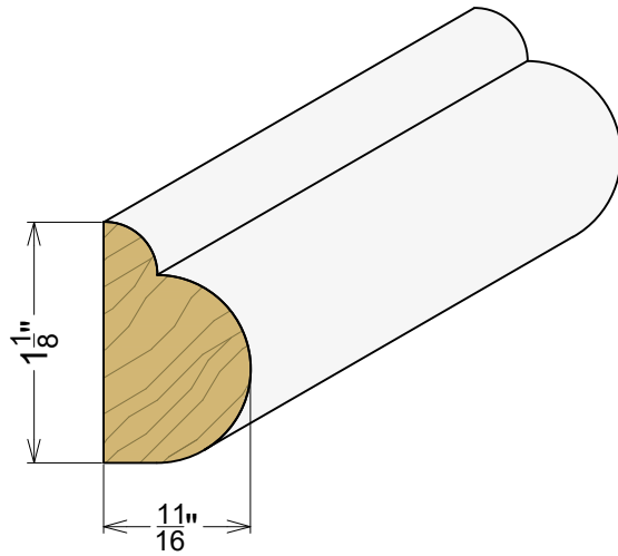
AP 6291 11/16" x 1-1/8"
