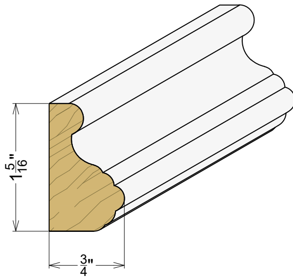
AP 6297 3/4" x 1-5/16"
