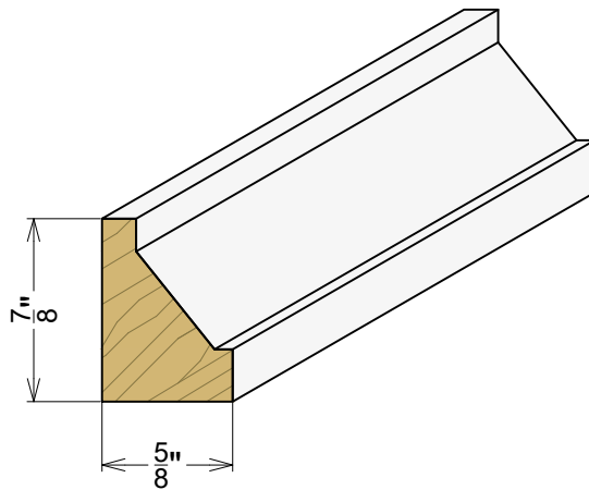
AP 6361 5/8" x 7/8"
