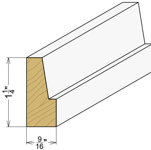
AP 6383 9/16" x 1-1/4"
