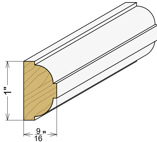
AP 6433 9/16" x 1"
