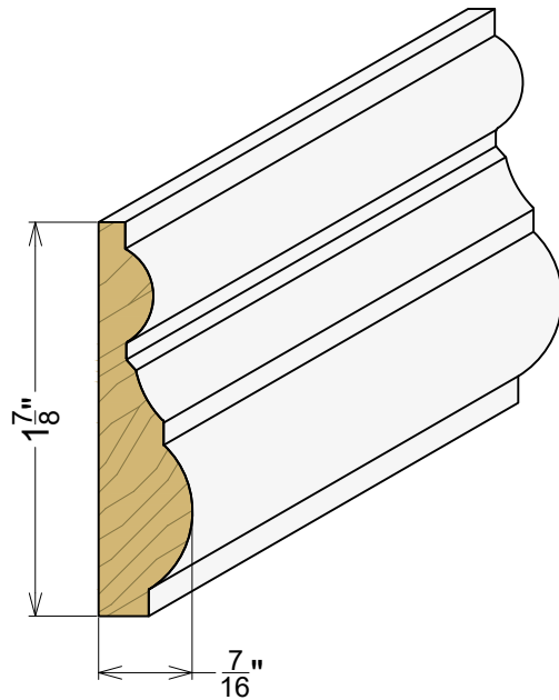
AP 6447 7/16" x 1-7/8"
