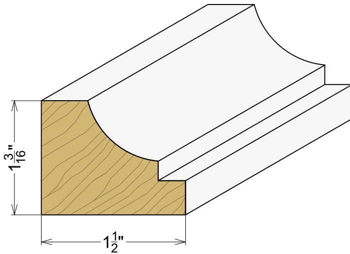
AP 6457 1-3/16" x 1-1/2"
