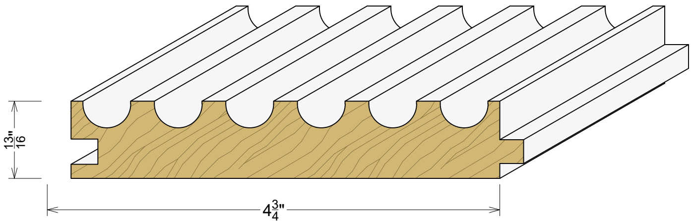
AP 6474 13/16"x 4 3/4"
