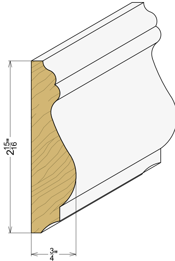
AP 7009 3/4" x 2-15/16"
