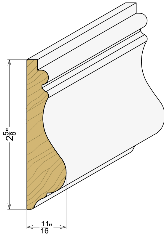
AP 7015 11/16" x 2-5/8"
