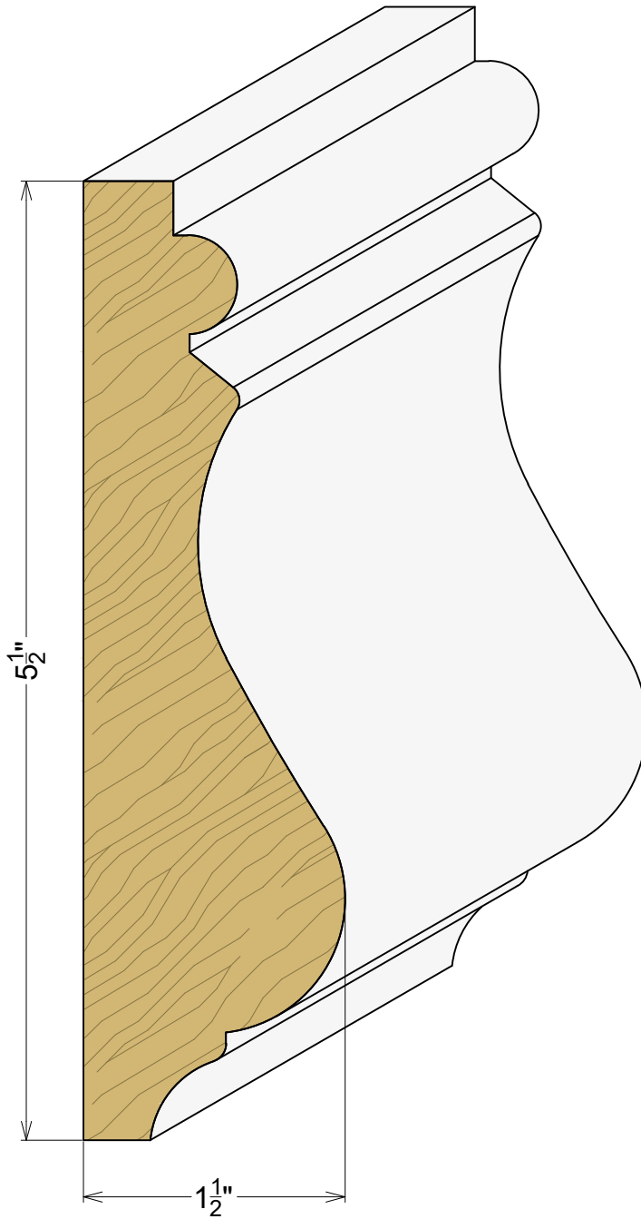
AP 7021 1-1/2" x 5-1/2"
