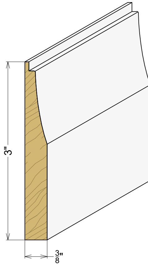
AP 7034 3/8" x 3"
