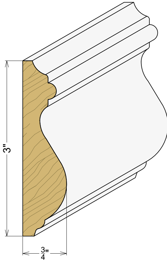
AP 7042 3/4" x 3"
