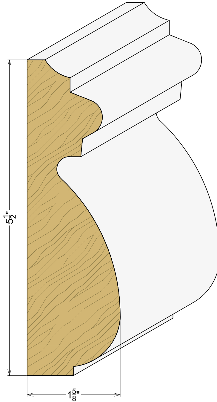
AP 7049 1-5/8" x 5-1/2"
