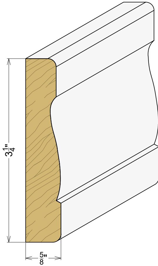
AP 7054 5/8" x 3-1/4"
