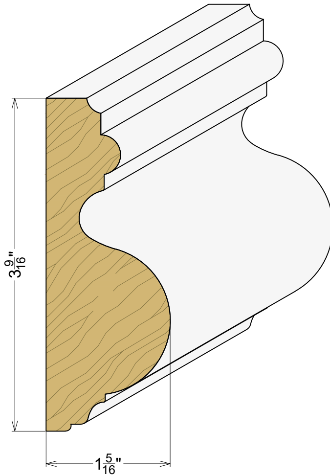
AP 7074 1-5/16" x 3-1/2"
