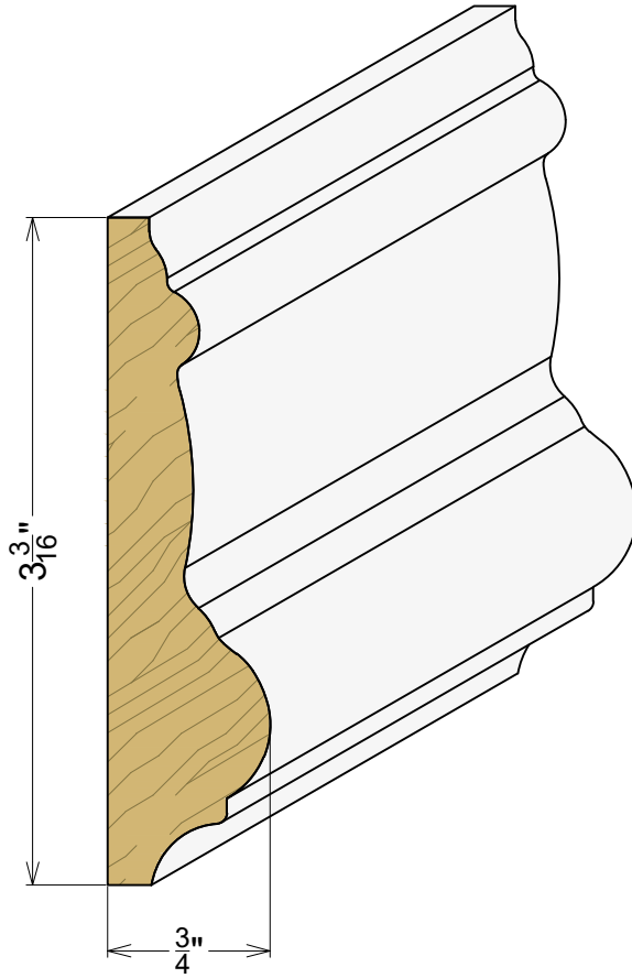
AP 7079 3/4" x 3-3/16"
