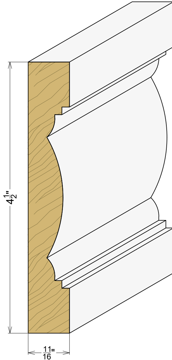
AP 7100 1 1/16" x 4-1/2"
