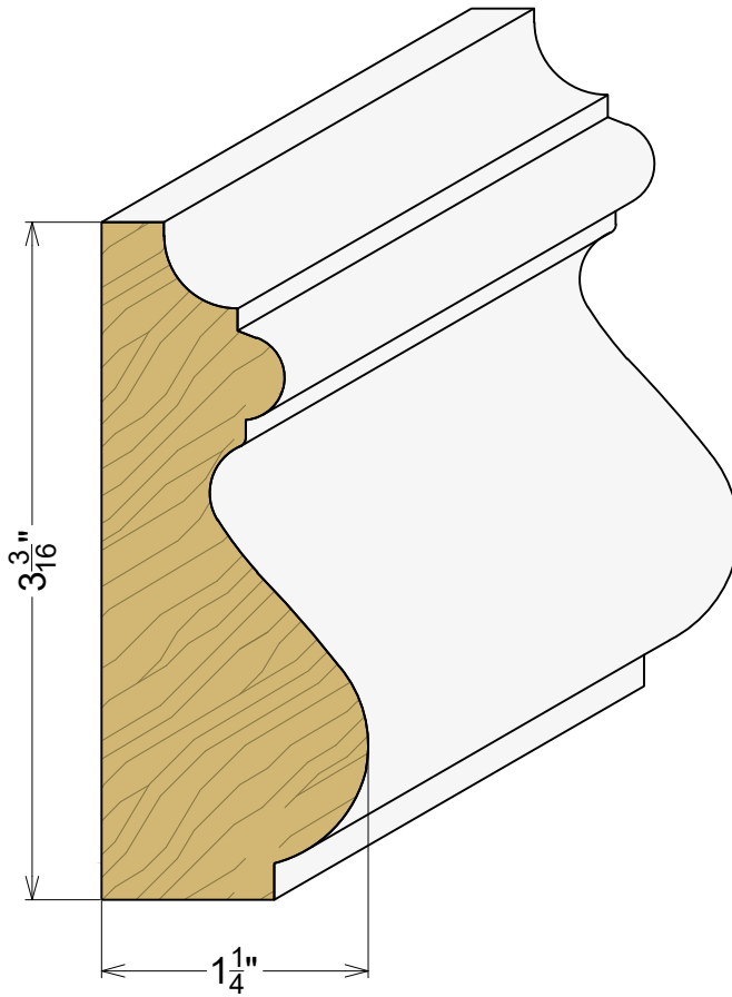
AP 7106 1-1/4" x 3-3/16"
