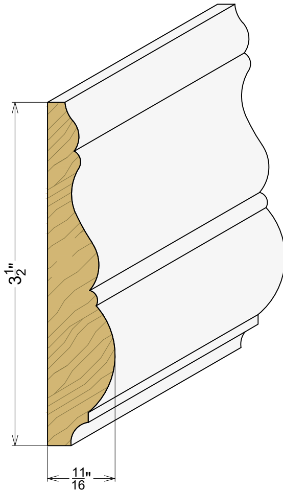
AP 7112 11/16" x 3-1/2"
