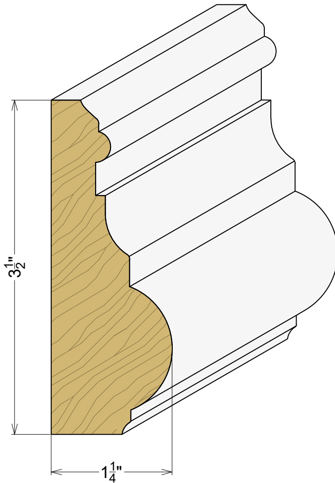
AP 7146 1-1/4" x 3-1/2"
