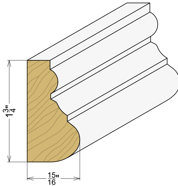
AP 7161 15/16" x 1-3/4"
