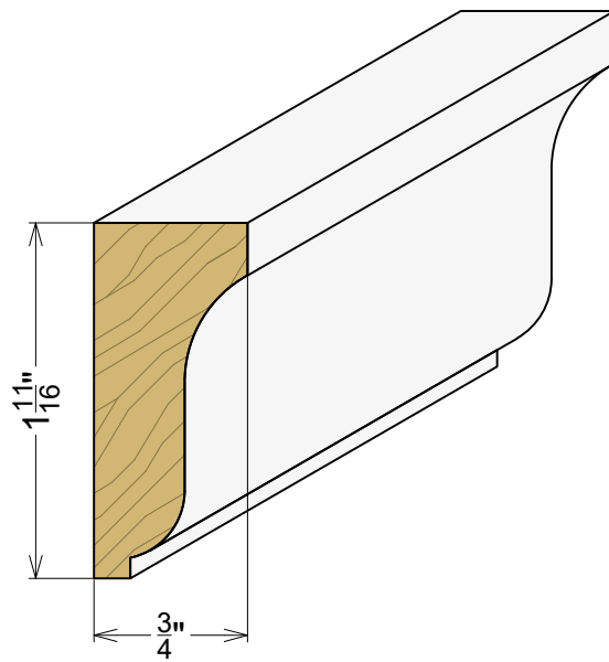
AP 7171 3/4" x 1-11/16"
