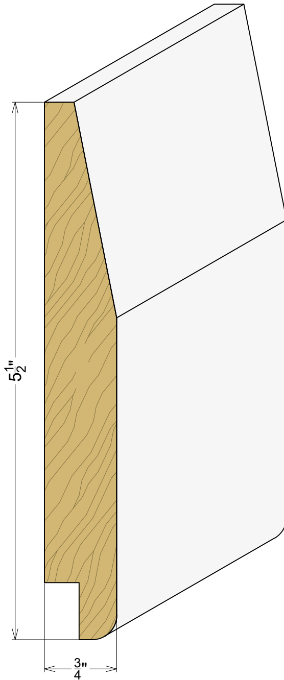
AP 8014 3/4" x 5-1/2"
