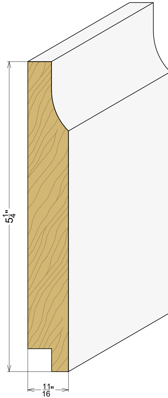
AP 8020 11/16" x 5-1/4"
