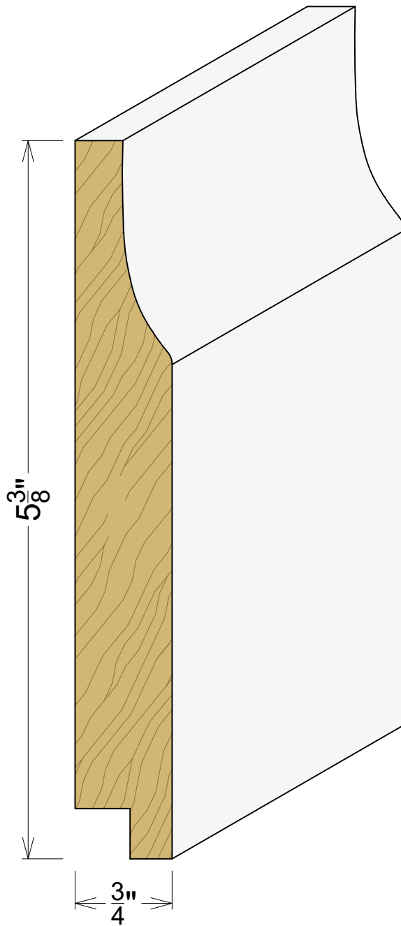
AP 8033 3/4"x 5 3/8"
