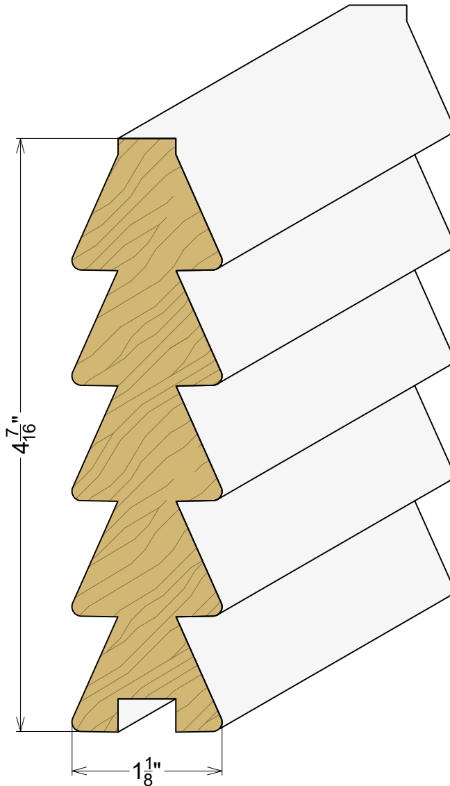
AP 9001 1-1/8" x 4-1/2" False Louver
