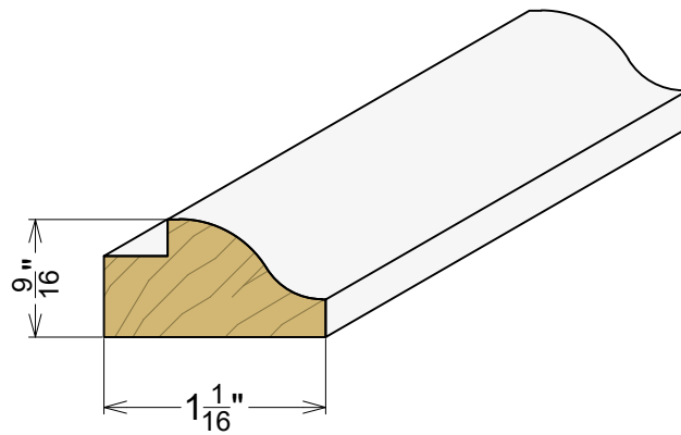
AP 9004 9/16" x 1-1/16" Applied Stop
