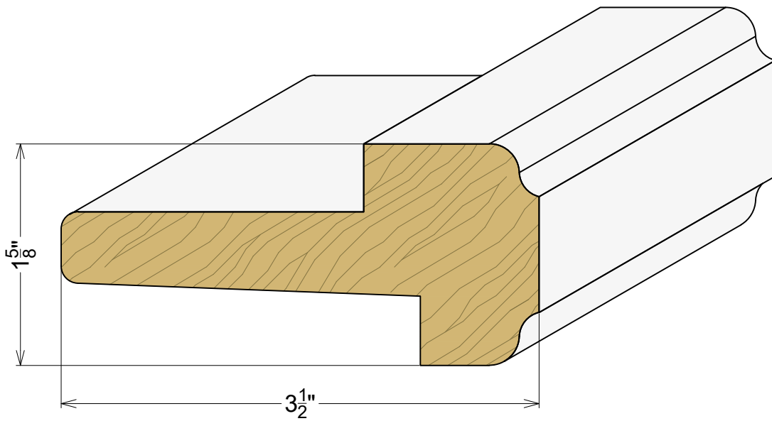
AP 9005 1-5/8" x 3-1/2"
