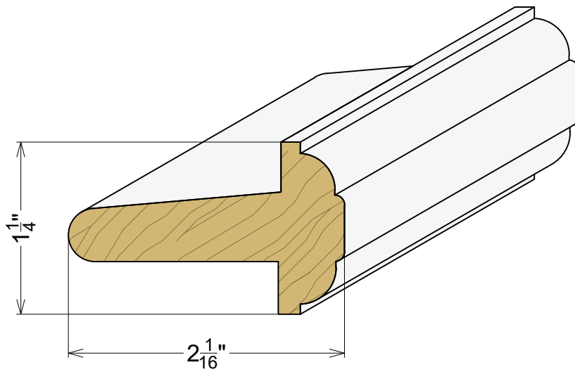
AP 9007 1-1/4" x 2-1/16"
