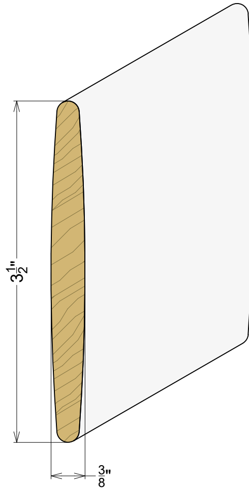
AP 9027 3/8" x 3-1/2" Plantation Louver
