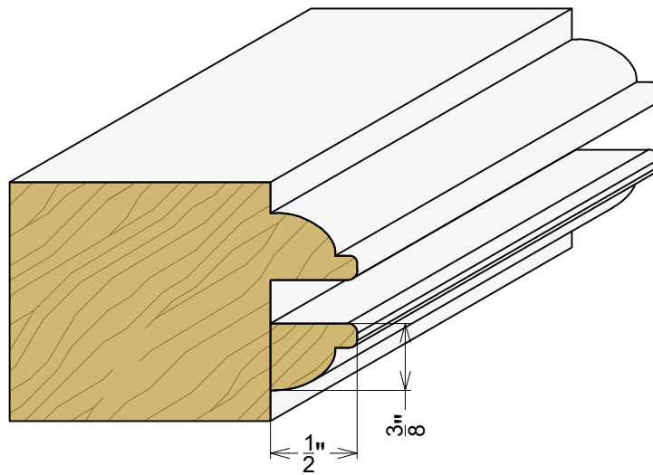
AP 9030 3/8" x 1/2" Profile Applied Stop
