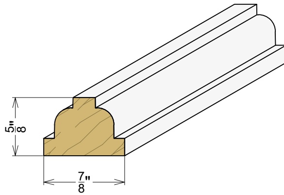
AP 9041 M 5/8" x 7/8" Profile
