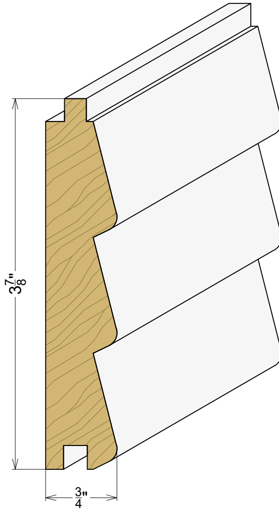
AP 9042 3/4" x 3-7/8" False Louver
