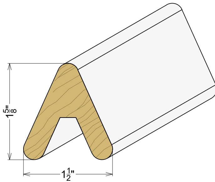
AP 9049 1-5/8" x 1-1/2" Two-Sided Louver
