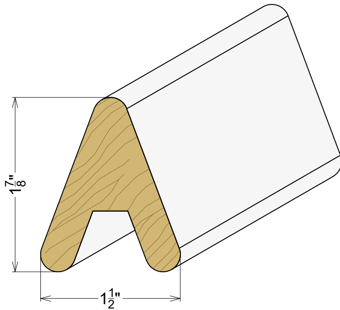
AP 9050 1-7/8" x 1-1/2" Two-Sided Louver
