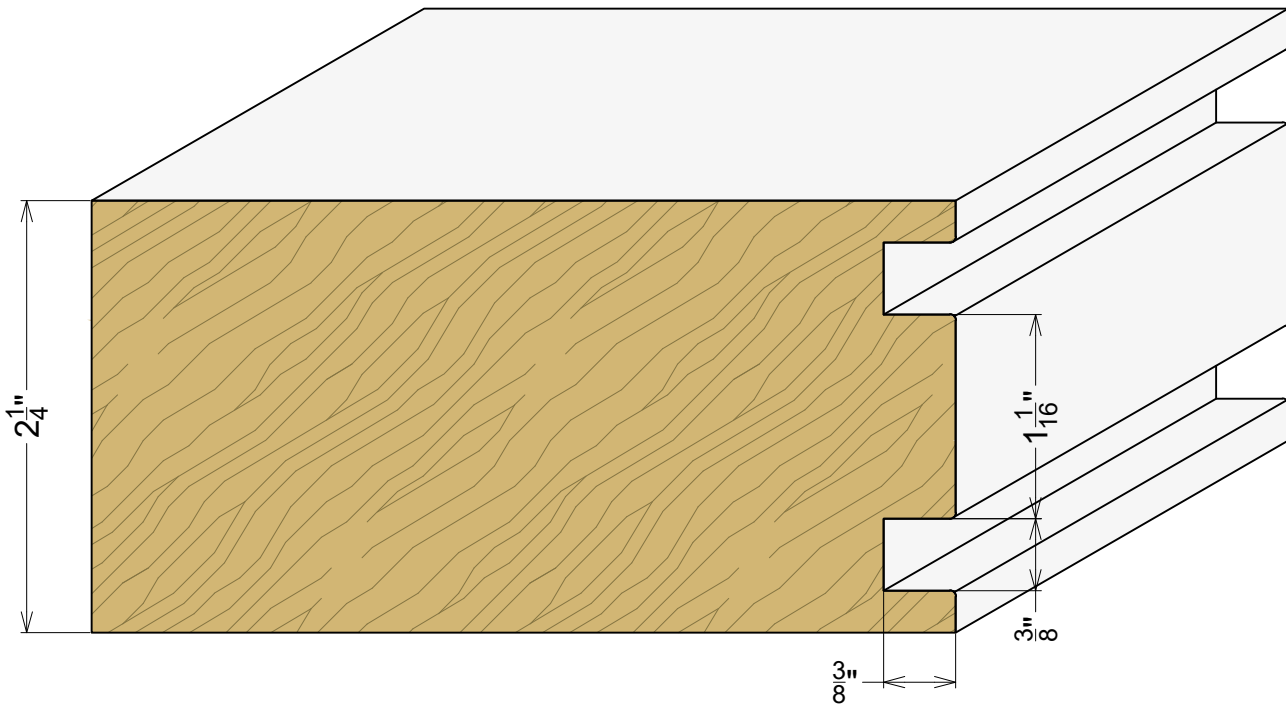
AP 9057B Double Applied Stop Door Profile 3/8" x 3/8" Grooves
