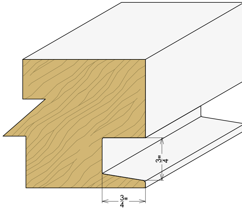
AP 9060-B 3/4" x 3/4" Profile 2-1/4" Door Profile
