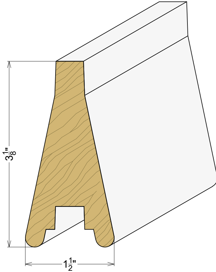
AP 9061 1-1/2" x 3-1/8" Two-Sided Louver
