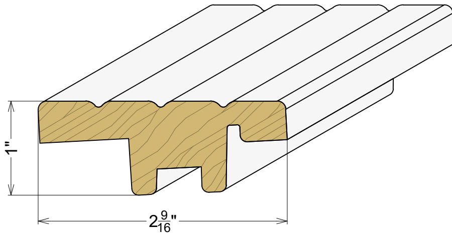
AP 9062 1" x 2-9/16" Threshold Top
