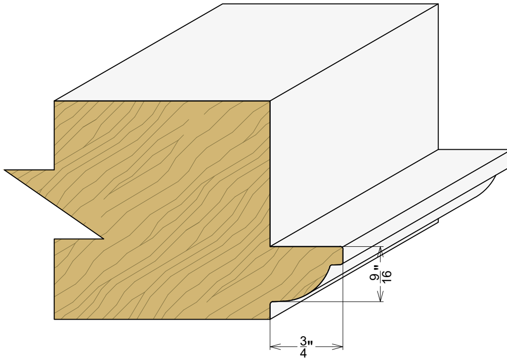
AP 9070 2-1/4" Door Profile
