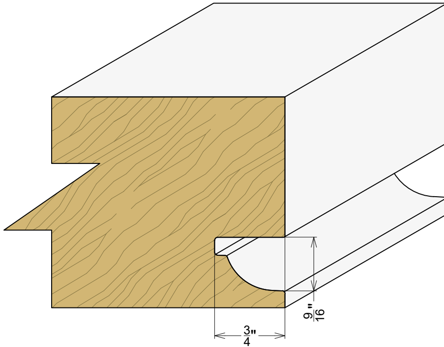
AP 9071 2-1/4" Door Profile
