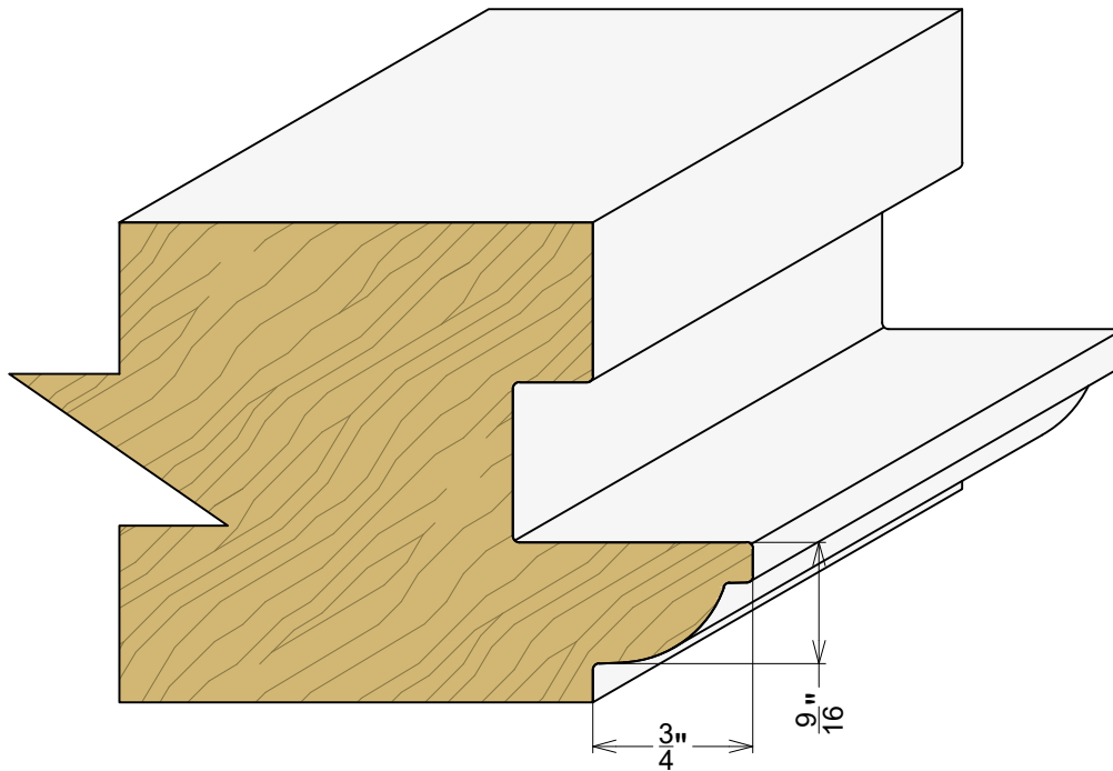
AP 9072 2-1/4" Door Profile
