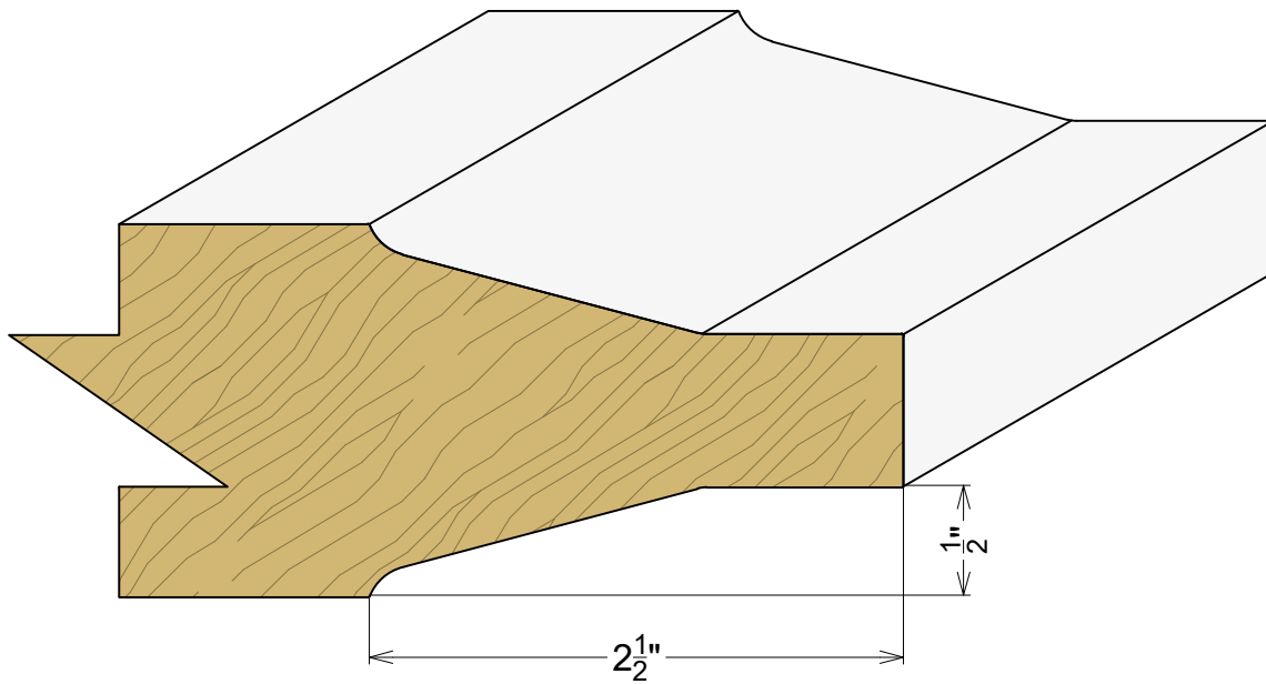
AP 9076 1-3/4" Panel Profile
