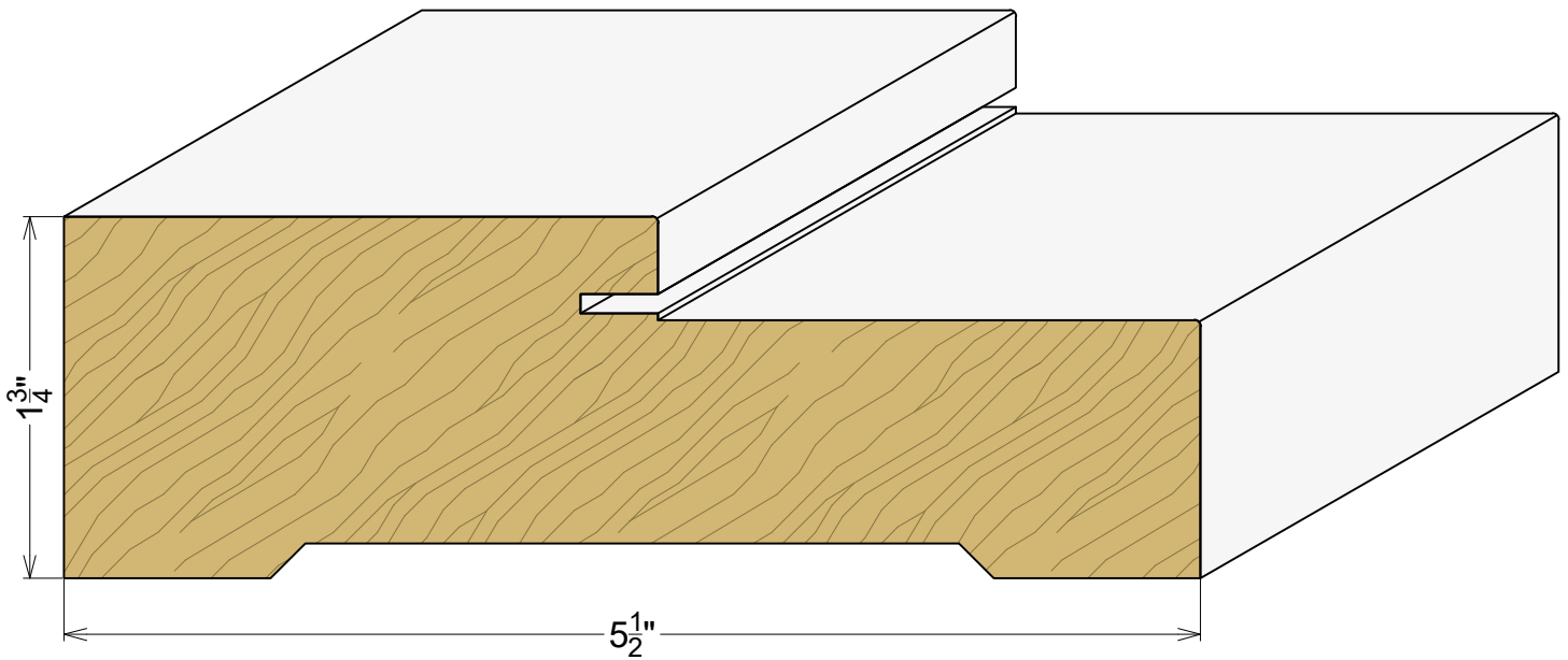
AP 9077 Jamb for 2-1/4" Doors
