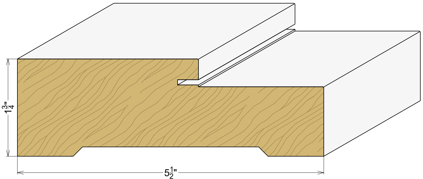
AP 9078 Jamb for 2-1/4" Sidelite
